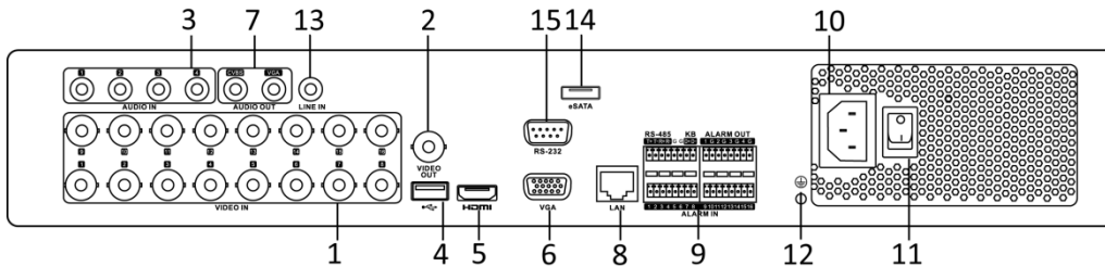
Figure 1-14 Rear Panel of DS-7300HQHI-K
